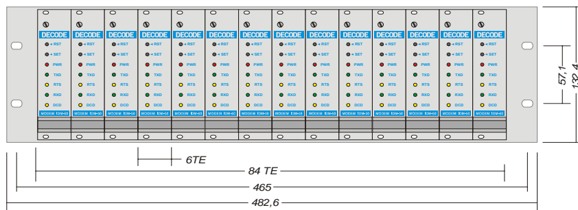
3U rack version with 14 modems per rack
